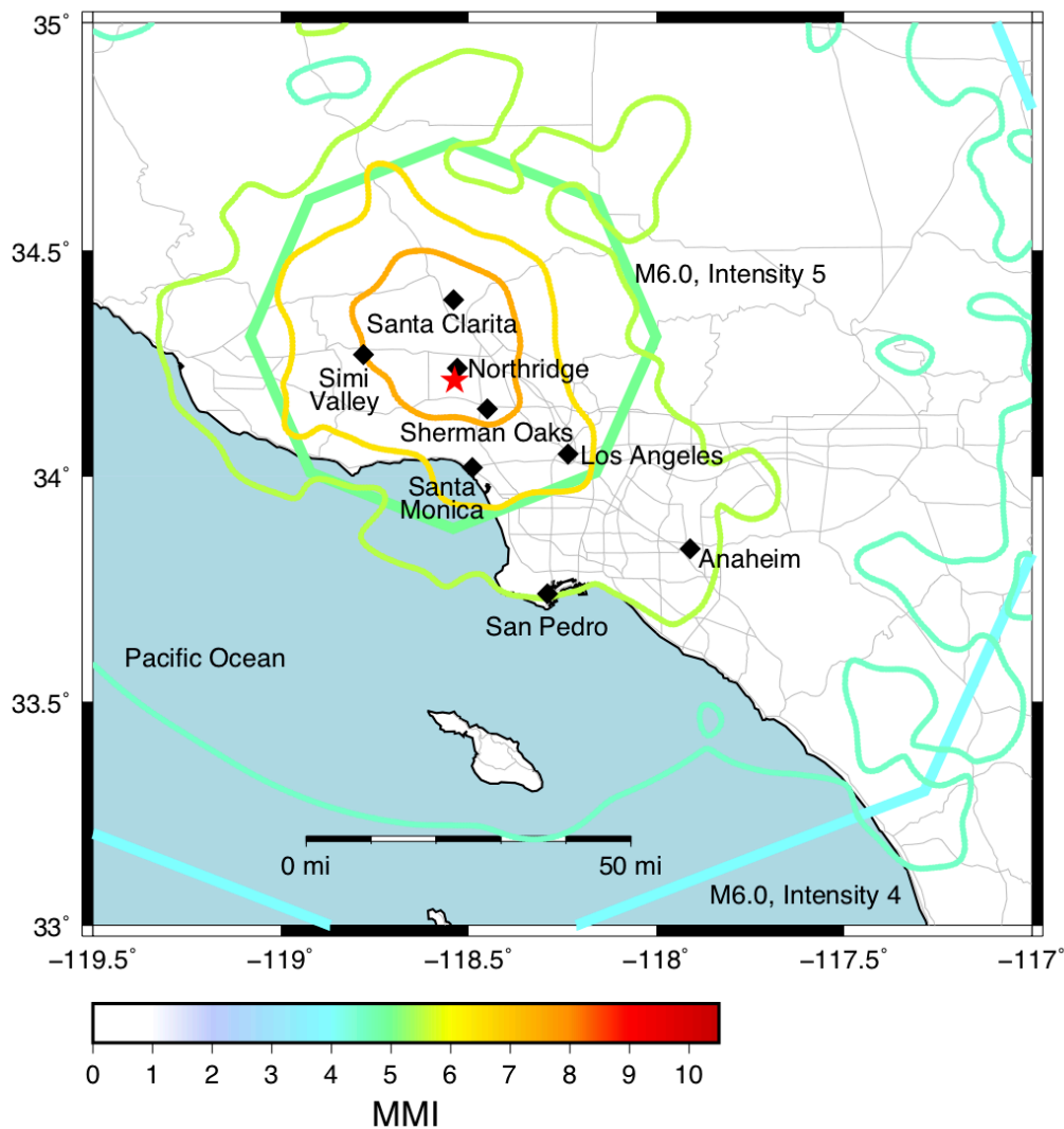
Figure 1. Contours of shaking in the 1994 Northridge Earthquake from the USGS ShakeMap ( Details available here ). Contours are given in Modified Mercalli Intensity (MMI) levels 4.5, 5.5, 6.5, and 7.5. The locations of cities discussed in the text are shown as labelled diamonds, the epicenter is shown as a red star. The extent of the area receiving alerts will grow during the initial seconds as the rupture expands over the fault and the estimate of earthquake magnitude increases. The initial magnitude estimate may be smaller (M5-6) than the final magnitude (6.7) and there may be errors in the real-time magnitude estimates. The green and light blue octagons denote the alerting regions for Android “take action” alerts (Intensity 5) and WEA (Intensity 4) when the magnitude estimate reaches 6.0 during the growing rupture. This indicates just one of multiple (expanding) alerts that would be sent out (see text). The Intensity 3 octagon, used by many cellphone apps, extends beyond the scale of this map.
