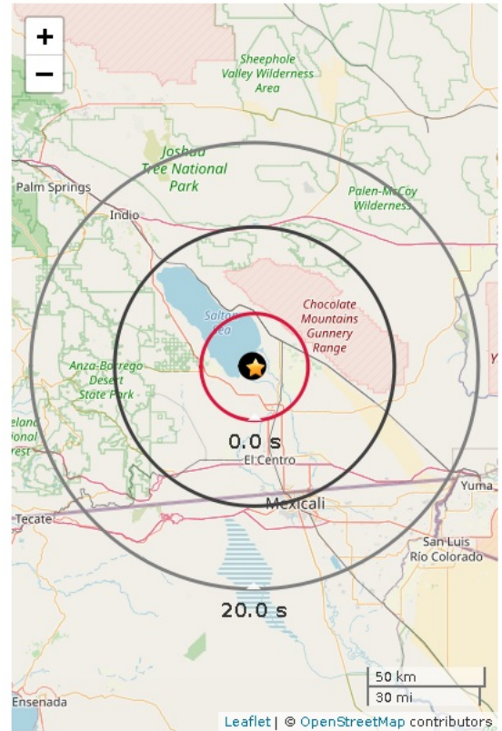
Figure 1. ShakeAlert initial earthquake location (black dot). Star is regional network epicenter. MMI 4 polygon is the estimated initial alert area. If shown***, red circle is front of peak shaking when the alert was released. Shaking takes 10 s to expand from circle to circle.
