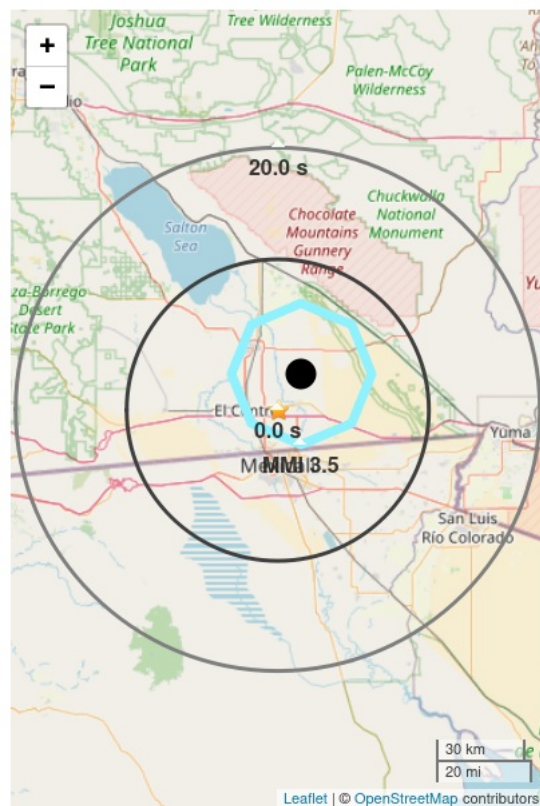
Figure 1. ShakeAlert initial earthquake location (black dot). Star is ANSS earthquake epicenter. Polygon shows the MMI 3.5 shaking intensity area. If shown, red circle is front of peak shaking when the Message was released***. Shaking takes 10 s to expand from circle to circle.
