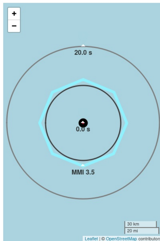
Figure 1. Initial earthquake locations from ShakeAlert (black dot). Polygon shows estimated area of MMI 3.5 and greater ground shaking**. Red circle (if shown) marks the position of the peak shaking wavefront at the time the Alert Message was issued***. Note, shaking takes 10 seconds to expand from circle to circle.
