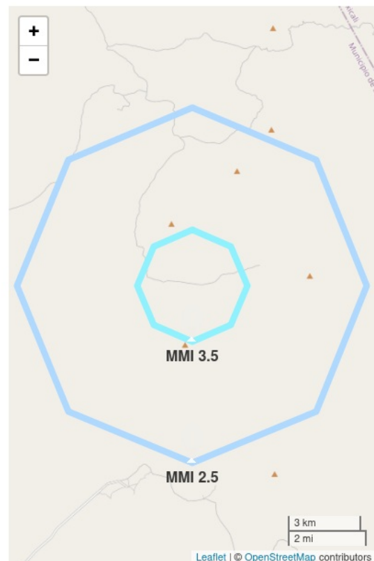
Figure 2. Polygons show the maximum estimated extent of ground shaking for different MMI** ranges (color-coded and labeled). Shaking of MMI 3 or less is often not felt. ANSS earthquake epicenter not available.
