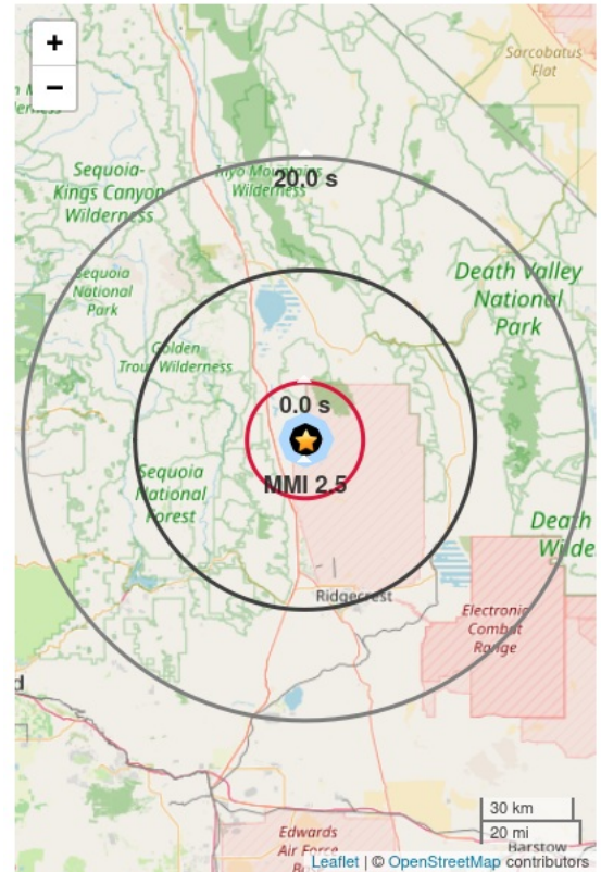
Figure 1. Initial earthquake locations from ShakeAlert (black dot) and ANSS (orange star). Polygon shows estimated area of felt ground shaking**. Red circle (if shown) marks the position of the peak shaking wave front at the time the Alert Message was issued***. Note, shaking takes 10 seconds to expand from circle to circle.
