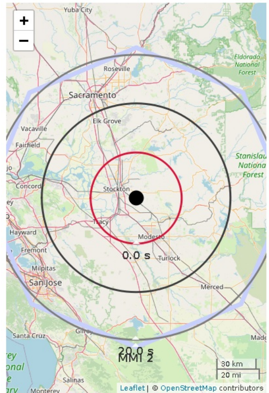
Figure 1. ShakeAlert initial earthquake location (black dot). Regional network epicenter not available. Polygon is the approximate outer range for felt ground motion. If shown***, red circle is front of peak shaking when the alert was released. Shaking takes 10 s to expand from circle to circle.
